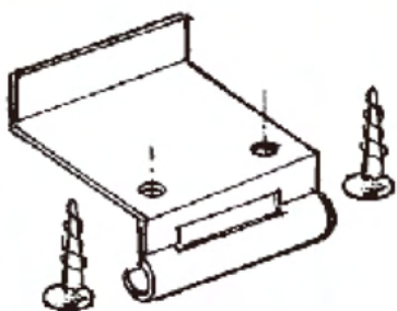
Guiding plate
