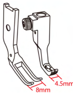
Narrow standard feet
