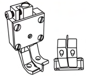
Compensating foot with a center guide on right toe
