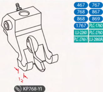
Pneumatic center guiding foot with extremely short toes Ⓢ KP768-YI
