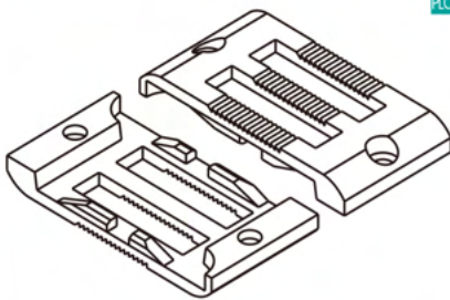
Needle plate for PLC-2760 PLC-2760
