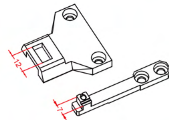
Raised, small needle plate & feed dog
