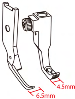
Narrow right cording feet
