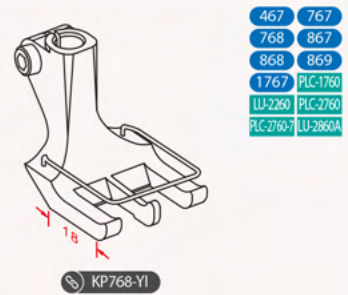
Fixed guiding foot with short toes Ⓢ KP768-YI
