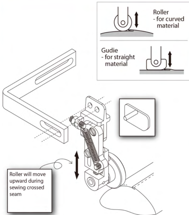
Left compensating roller guide
