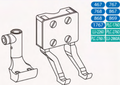
Double needle compensating feet set
