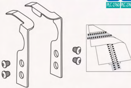
Downturn hemmer attachment
