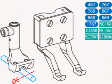
Double needle compensating feet for piping
