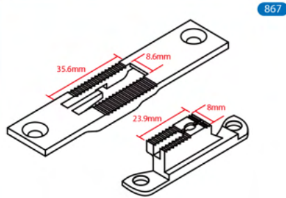
Needle plate & feed dog for thin material
