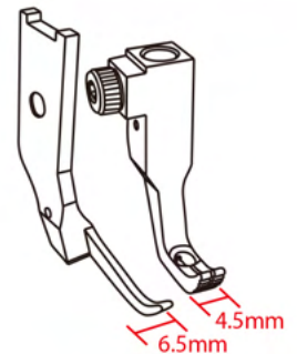
Narrow left cording feet
