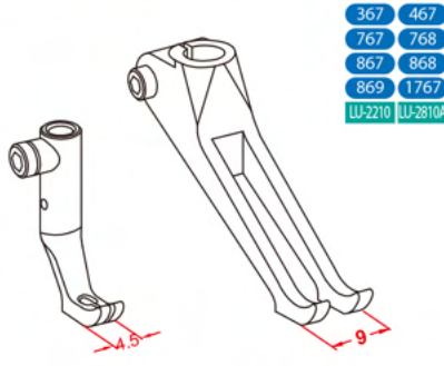
Narrow standard feet
