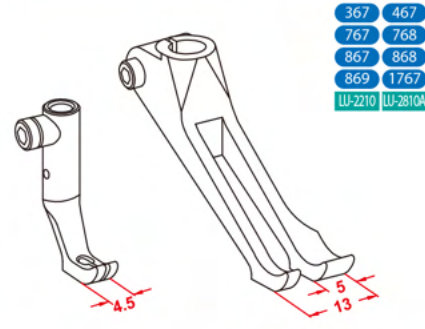
Narrow standard feet with wider right toe
