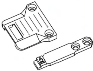
Standard needle plate & feed dog
