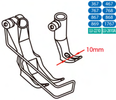
Wider standard feet
