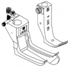
Stronger right compensating guide & wider feeding foot for HEAVY DUTY
