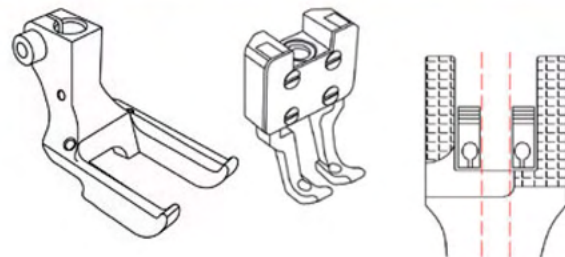
For center cording/piping
