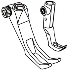
Presser foot width : 10mm Feeding foot width : 4.5mm Narrow standard feet
