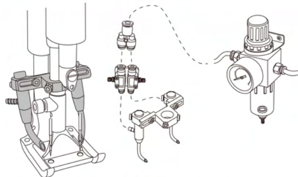
Needle cooler for double needle machine
