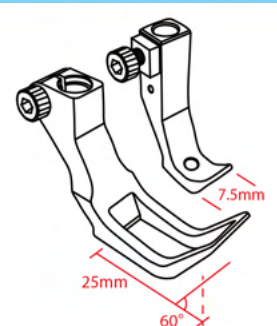
Climbing over thicker materials
