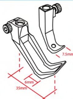
Climbing over cross seams
