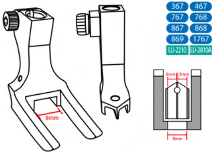
Presser feet for invisible zipper
