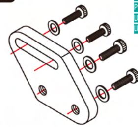
Mounting bracket
