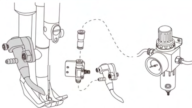
Needle cooler for single needle machine
