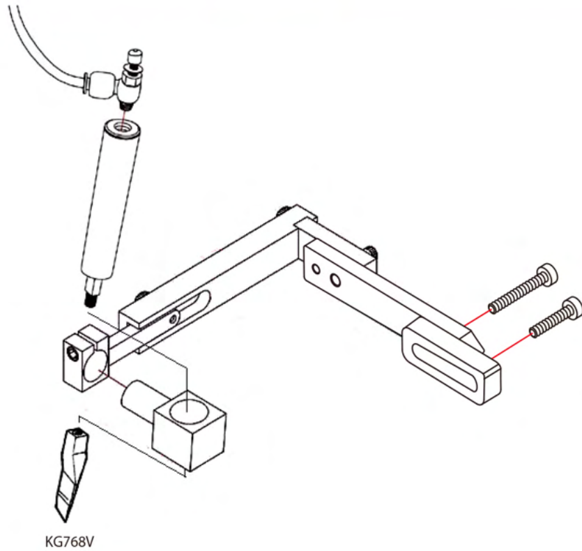
Pneumatic guiding set
