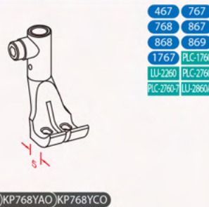
Short toes feeding foot Ⓢ KP768YAO KP768YCO
