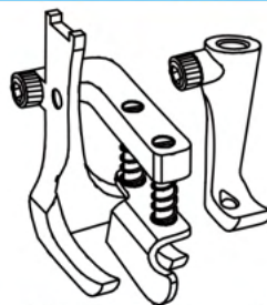
Deeper right compensating guide with balancing spring for EXTREME HEAVY DUTY
