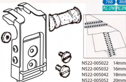
Belt guide with downturn hemmer
